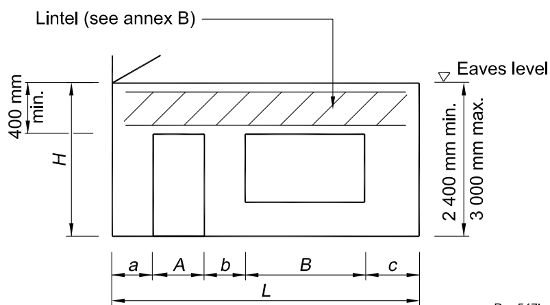
a) Wall with door and window openings
