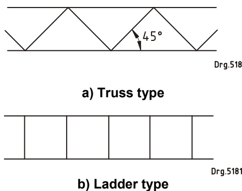
Figure 1 — Brickforce types
