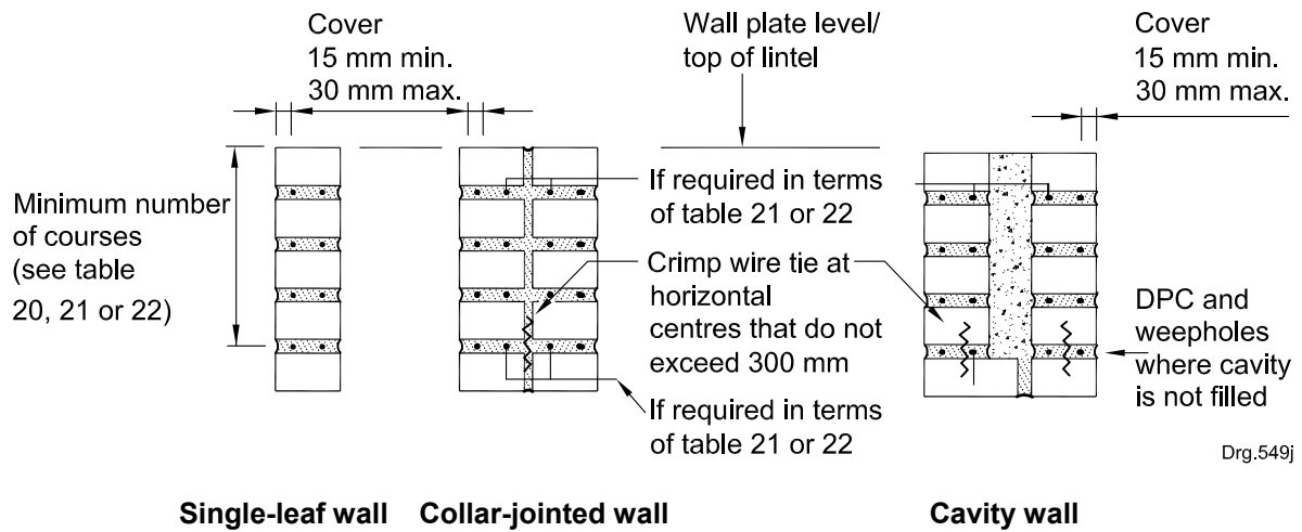
a) Typical section through lintel
