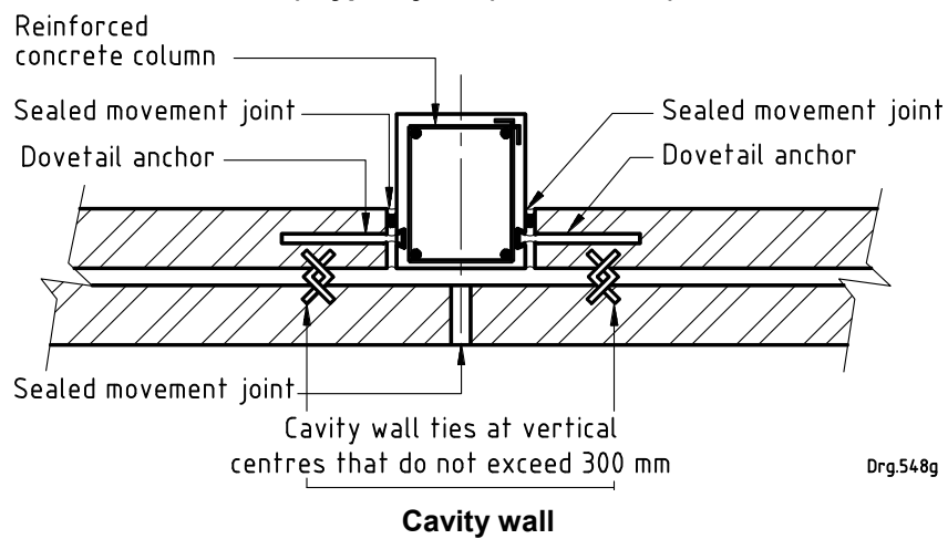
d) Type II joint (alternative 2)
