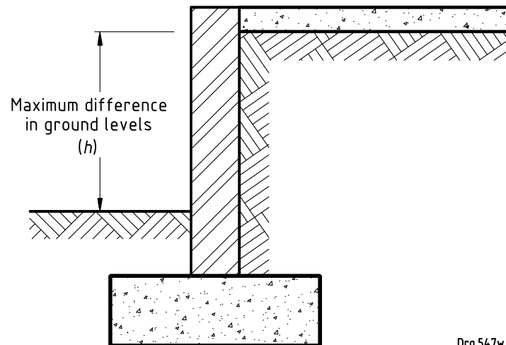
Figure 9 — Foundation walls
