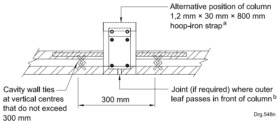
c) Fixing detail for cavity walls (type I or type II joint)
