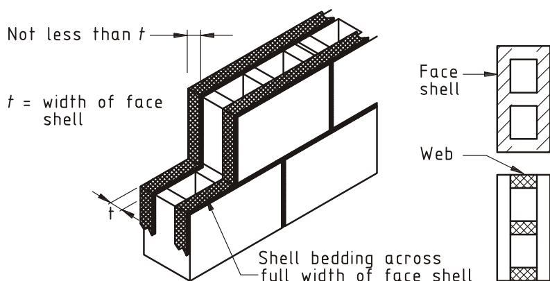
Figure 3 — Shell bedding
