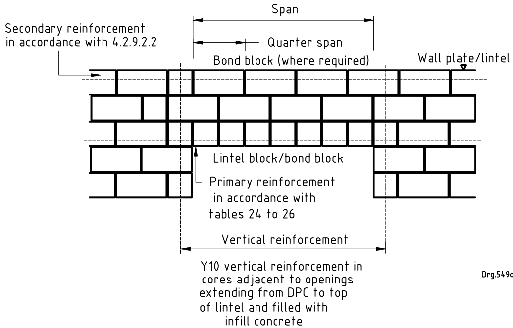
a) Single opening
