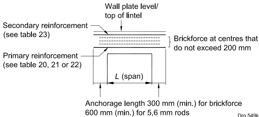
b) Single opening
