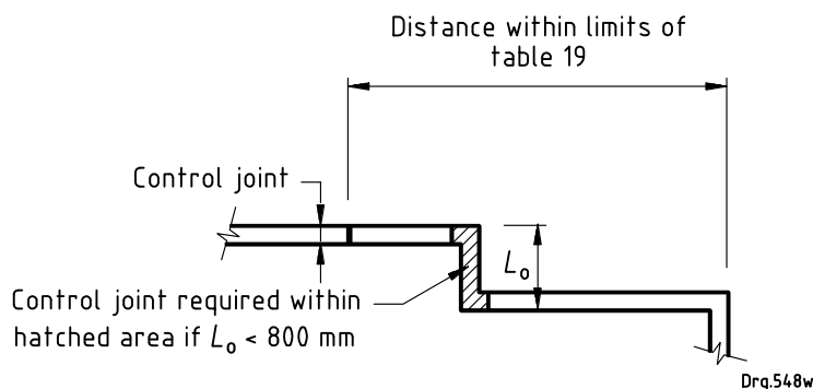
Figure 19 — Location of control joints in buildings
