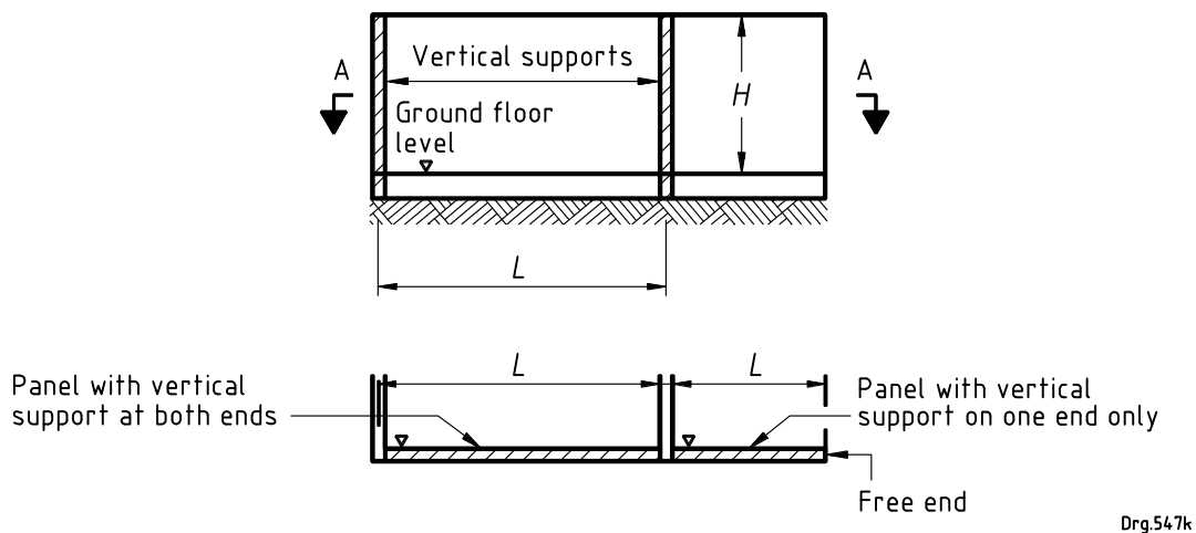
a) Panel proportions
