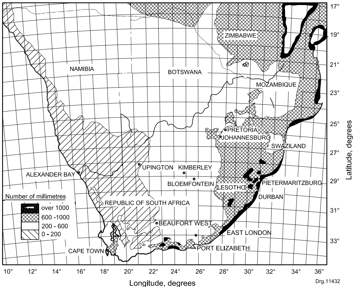
Figure C.2 — Mean annual rainfall
