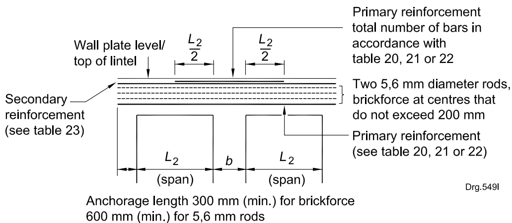
c) Openings with narrow pier where b < 750 mm
